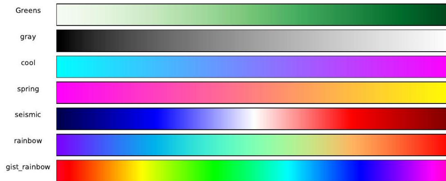
Figure 8.9: Color scales from Python's Matplotlib, varying hue, saturation, and brightness. Rainbow color maps are perceptually non-linear, making it difficult to recognize the magnitudes of differences.
