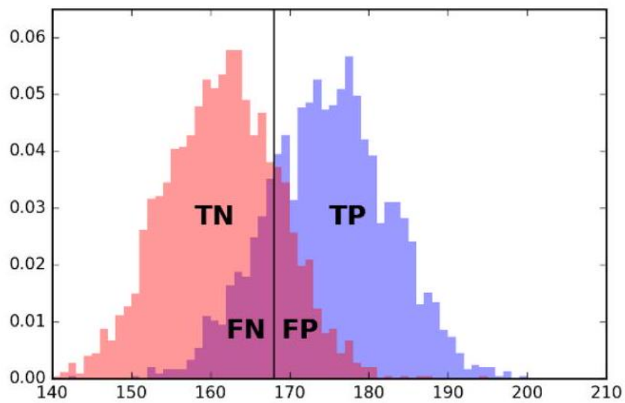
Figure 9.2: What happens if we classify everyone of height \geq 168 centimeters as male? The four possible results in the confusion matrix reflect which instances were classified correctly (TP and TN) and which ones were not (FN and FP).
