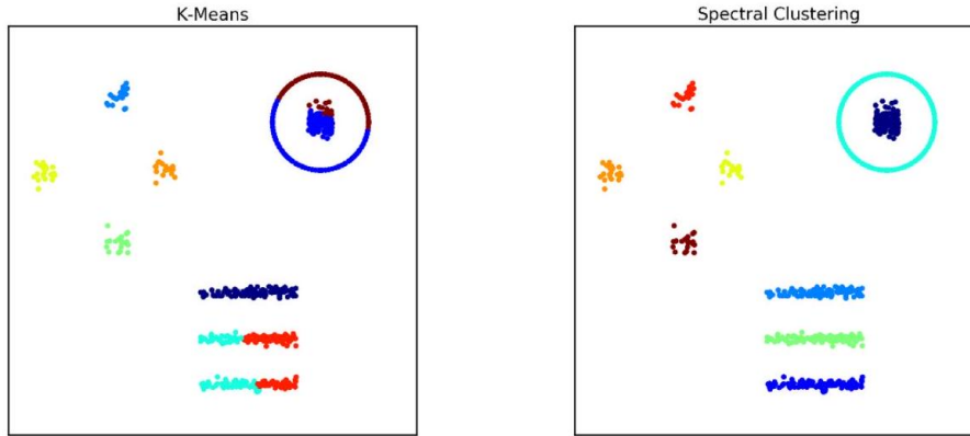
Figure 12.20: The results of k -means (left) and cut-based spectral clustering (right) on our 9-cluster example. Spectral clustering correctly finds connected clusters here that k -means cannot.
