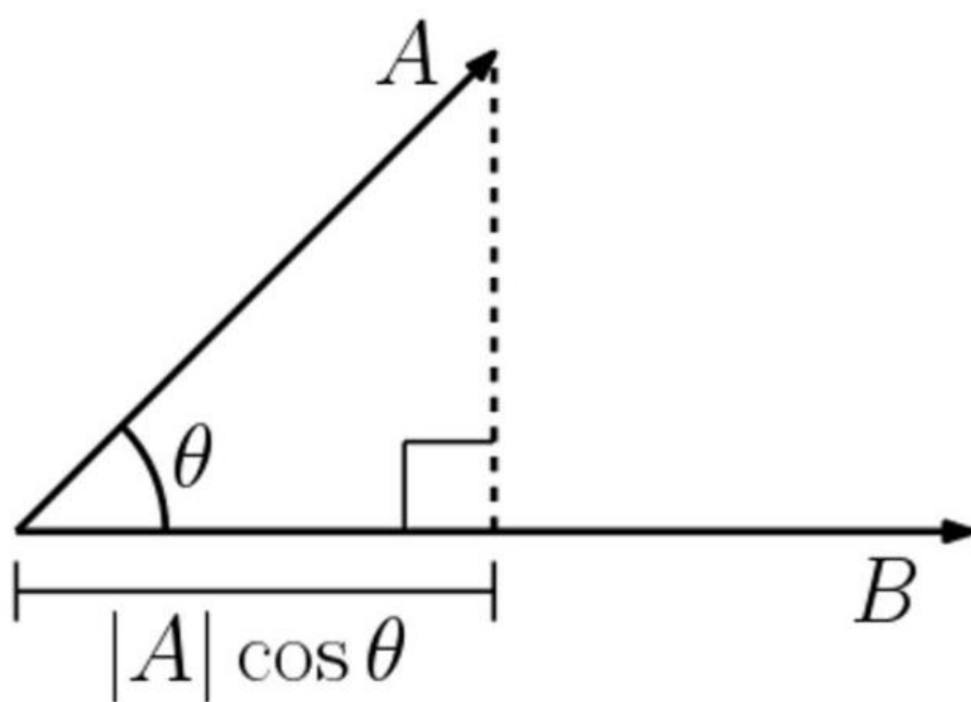
Figure 10.2: The dot product of two vectors defines the cosine of the angle between them.
