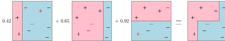
Figure 13.3: The final classifier is a weighted ensemble that correctly classifies all points, despite errors in each component classifier which are highlighted in red.
