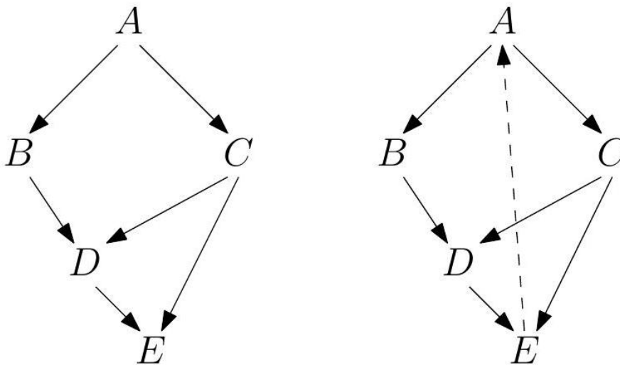
Figure 6.7: Consistently ordered preferences yield an acyclic graph or DAG (left). Inconsistent preferences result in directed cycles, which can be broken by deleting small sets of carefully selected edges, here shown dashed (right).
