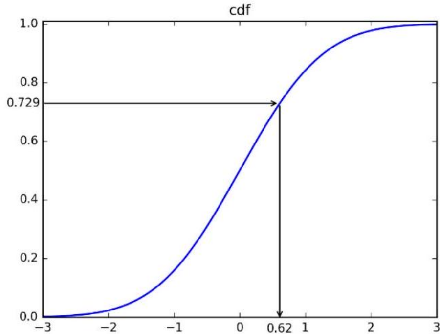
Figure 7.8: The inverse transform sampling method enables us to convert a random number generated uniformly from [0, 1] (here 0.729 ) to a random sample drawn from any distribution, given its cdf.
