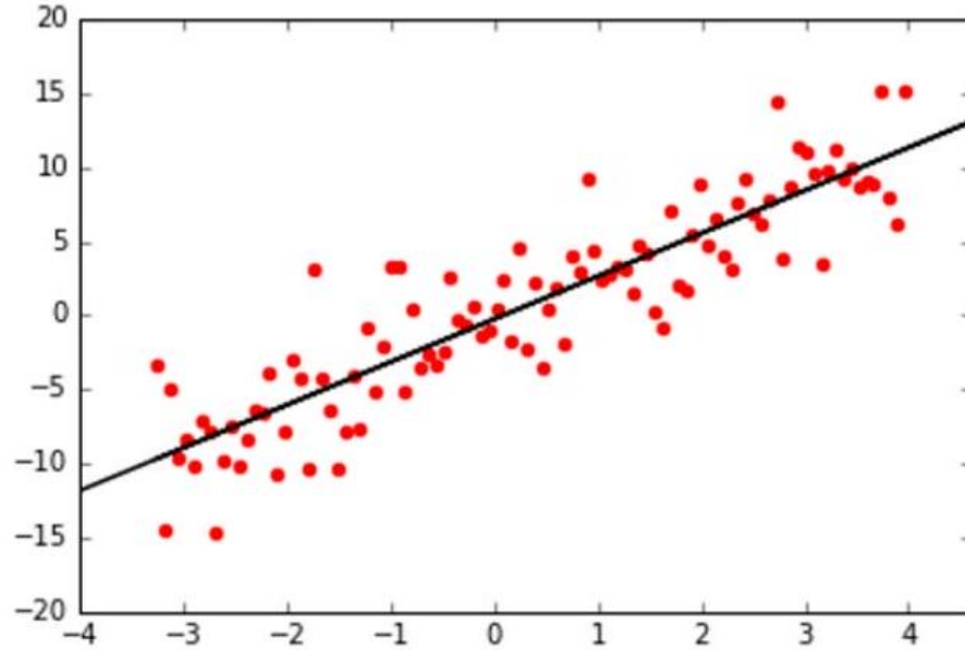
Figure 11.1: Linear regression produces the line which best fits a set of points.
