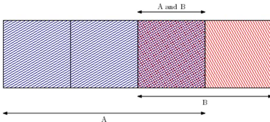
Figure 7.19: Bayes' Theorem in action.
