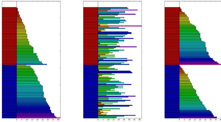
Figure 7.15: Permutation tests reveal the significance of the correlation between gender and the height (left). A random assignment of gender to height (center) results in a substantially different distribution of outcomes when sorted (right), validating the significance of the original relationship.
