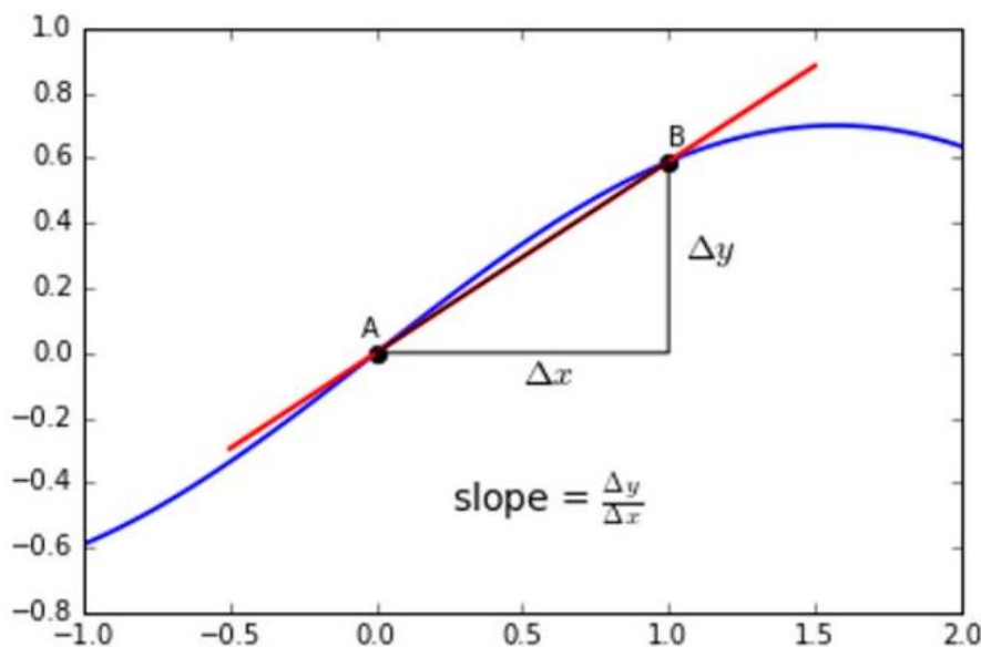
Figure 11.8: The tangent line approximates the derivative at a point.
