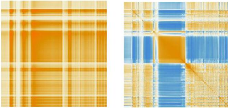
Figure 10.10: The Lincoln memorial's biggest eigenvector suffices to capture much of the detail of its covariance matrix.
